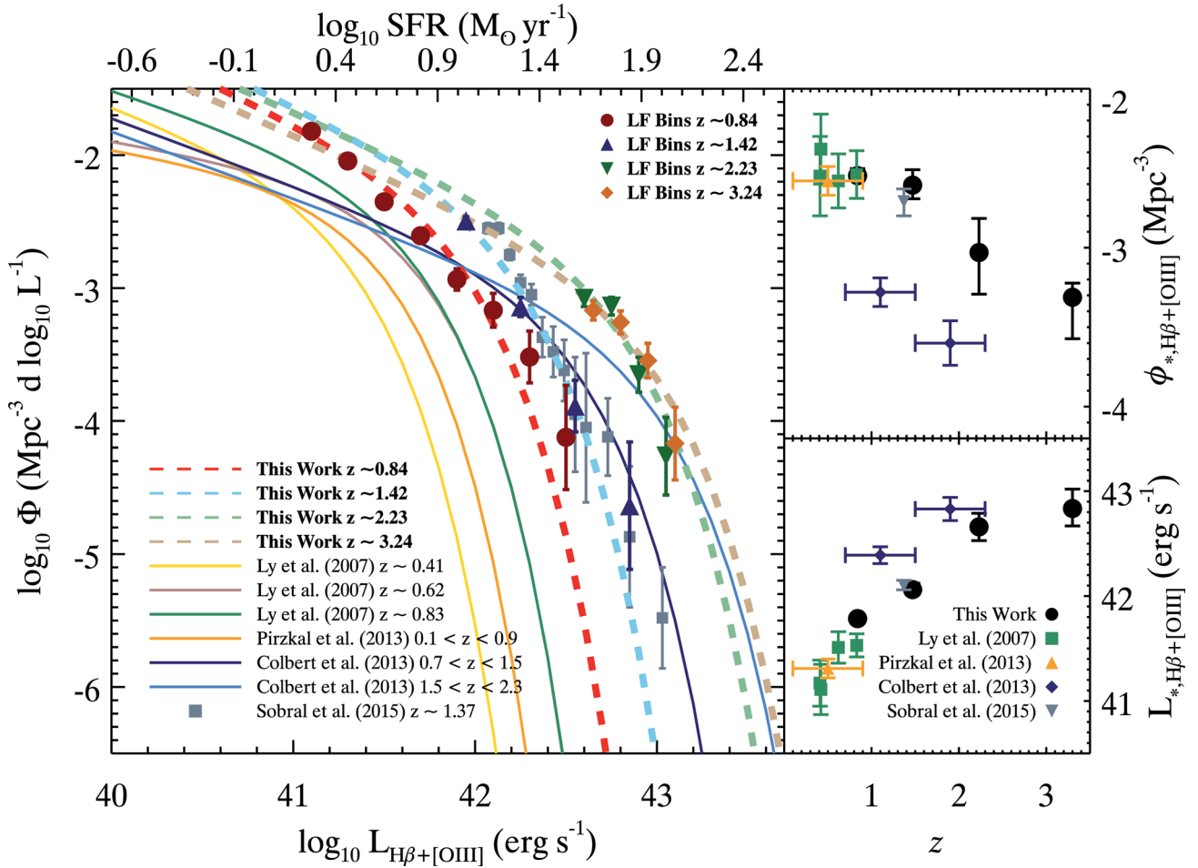
Figure 4. Left: presented are our H\beta + [O\text{III}] LFs along with LFs from the literature. Included on the top horizontal axis is the \log_{10} \text{SFR} that was derived via the Osterbrock & Ferland (2006) calibration (see Section 4.2). The darker data points are colour coded to match the lighter LF fit (dashed lines). There is a clear evolution in the LFs up to z \sim 3 . We find that our z = 1.42 and 2.23 LFs are in reasonable agreement with the [O\text{III}] grism spectroscopy study of Colbert et al. (2013) at the bright-end, suggesting that we are selecting a reliable sample of [O\text{III}] emitters. The major difference between our z = 0.84 and the z = 0.83 LF of Ly et al. (2007) is probably due to sample size biases. Our sample is much larger, hence we are able to populate our brightest bins, causing a shift in L_* to higher luminosities. Top right: the evolution of \phi_* from the H\beta + [O\text{III}] LF. A strong, decreasing evolution is seen in \phi_* from z = 0 to z \sim 3 . This same evolution is seen by UV LF studies (see Oesch et al. 2010 for details). Bottom right: the evolution of L_* from the H\beta + [O\text{III}] LF. We see a strong, increasing evolution in L_* up to z \sim 3 .
