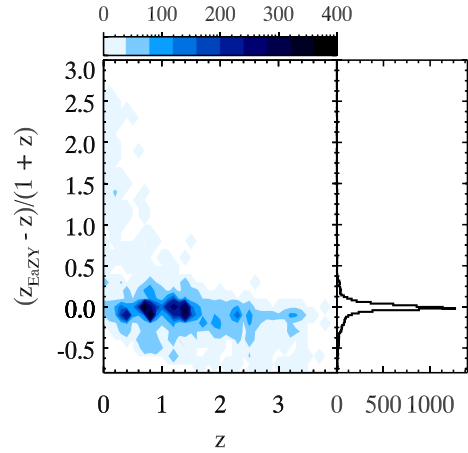
Figure 1. The 2D density distribution of the errors between the redshifts determined by EaZY and those of Ilbert et al. (2009, COSMOS, Le Phare) and Cirasuolo et al. (2007, UDS, Hyperz) for all narrow-band excess sources (full catalogue). We find that \sim 95 per cent of our measurements are in agreement with the redshifts from the literature. The median error is measured as 0.038 without sigma-clipping. There are overdensities at z \sim 0.4, 0.8 , and 1.5 that conform to redshifts for our major emission lines. We find outliers with errors up to \sim 2.5 , but these are only 4 per cent of our sample. In comparison to the wealth of spectroscopic data, we find a median photometric redshift error of \Delta z / (1 + z_{\text{spec}}) = 0.047 in comparison to spectroscopic redshifts.
